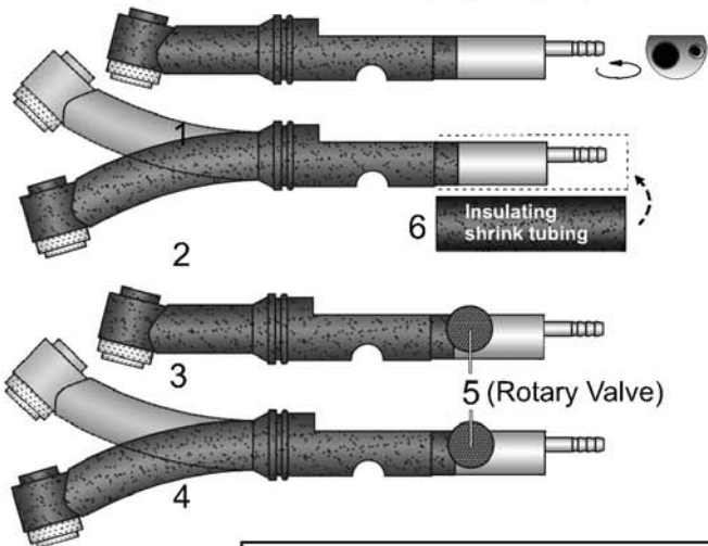
Forma WIG-handle with ball joint and different modular switch units
