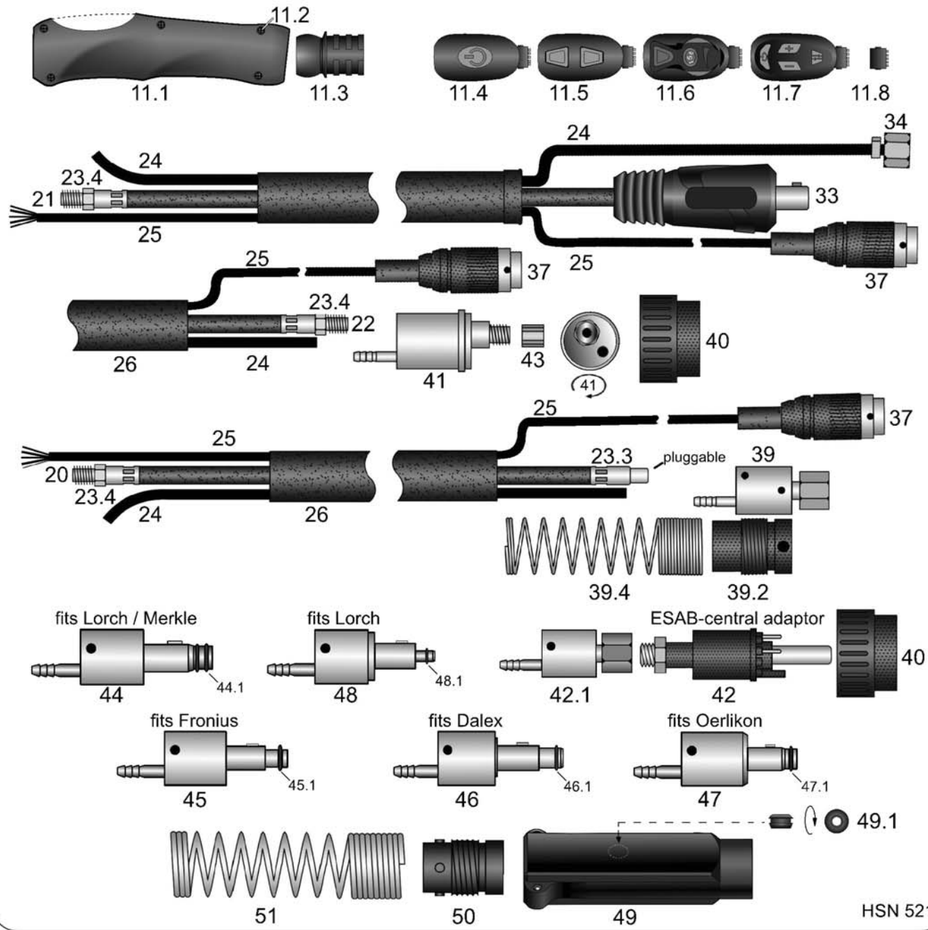
Forma WIG-handle with ball joint and different modular switch units
